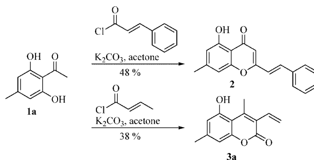
Scheme 1. Serendipitous formation of 3-vinylcoumarins.
