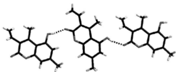
Figure 1. A fragment of crystal packing and hydrogen bonding scheme showing different orientations of the vinyl substituents in independent coumarin molecules A and B of 3a . Hydrogen bonds are indicated.
